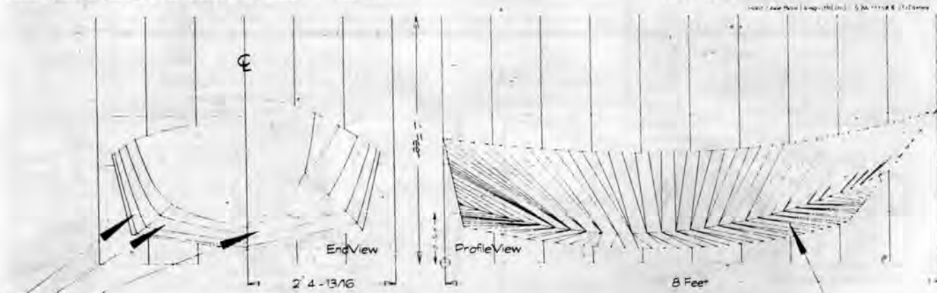
Figure 1. End View and Profile View of a small pram. Ruling lines describe surface of the panels of the hull in Profile. Station cross-sections in End View show how the intersections of the flexed panels with most stations and the transoms are curved.
