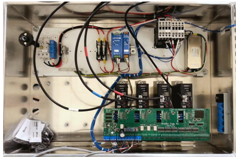
Control Box Interior
